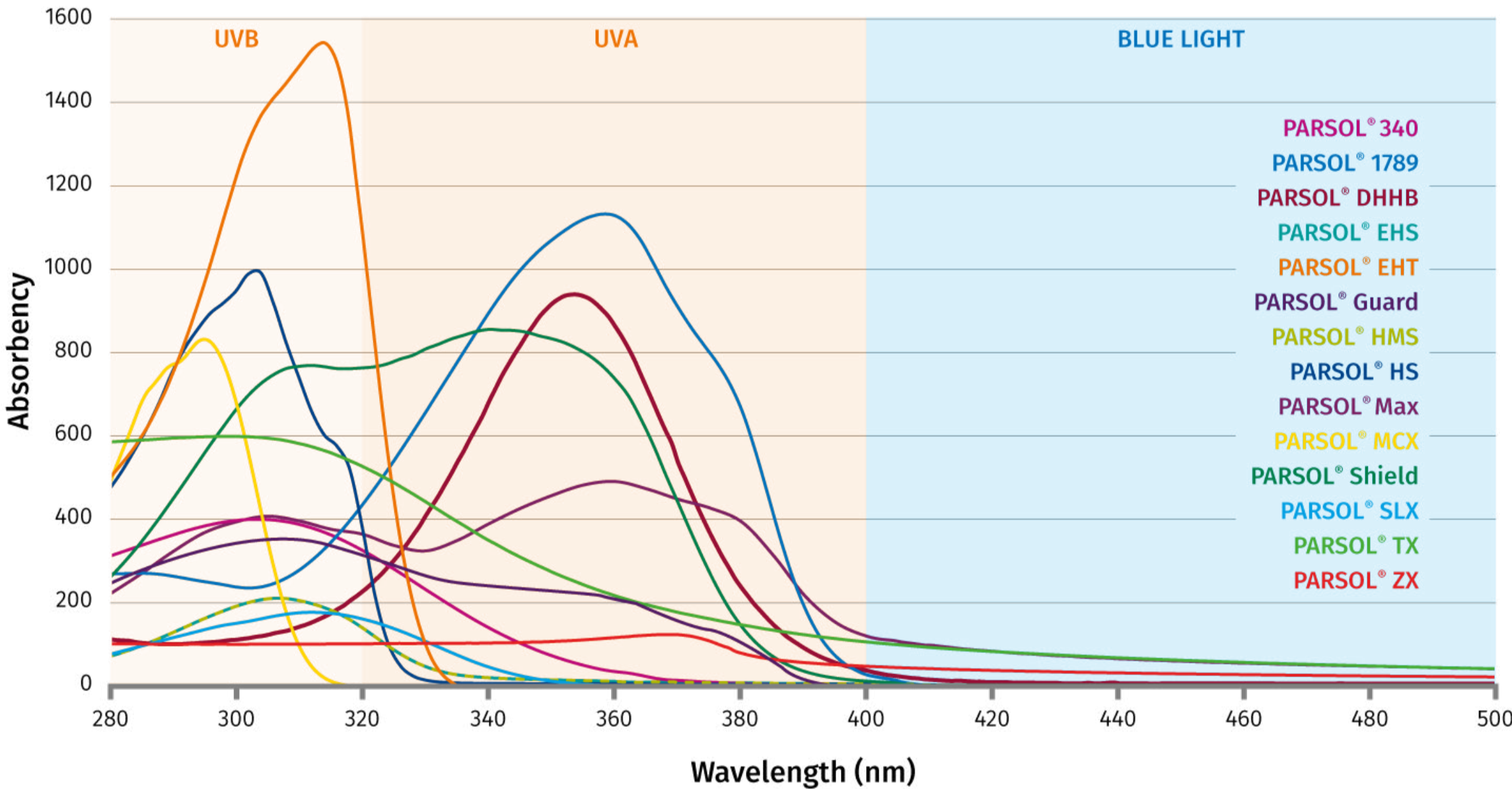
UV absorption spectrum of most commonly used UV-filters
